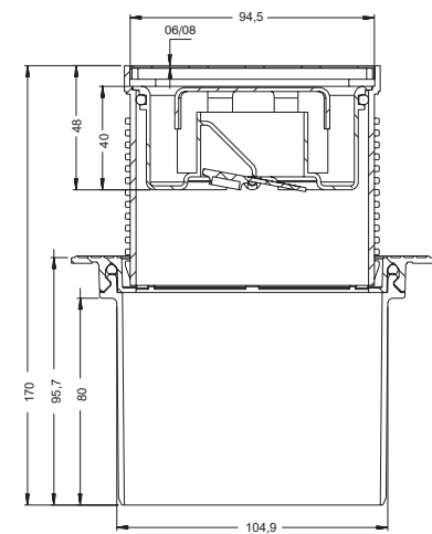
Ø 100 Vertical Outlet
